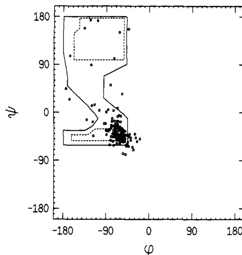
FIGURE 2: Plot of the main-chain dihedral angles. A Ramachandran plot of all non-glycinyl main-chain dihedral angles for the apoLp-III model is shown. Fully allowed \phi, \psi values are enclosed by dashed lines; those only partially allowed are enclosed by solid lines. As can be seen from consideration of just \phi, \psi values alone, the apoLp-III structure is almost entirely \alpha -helical.
